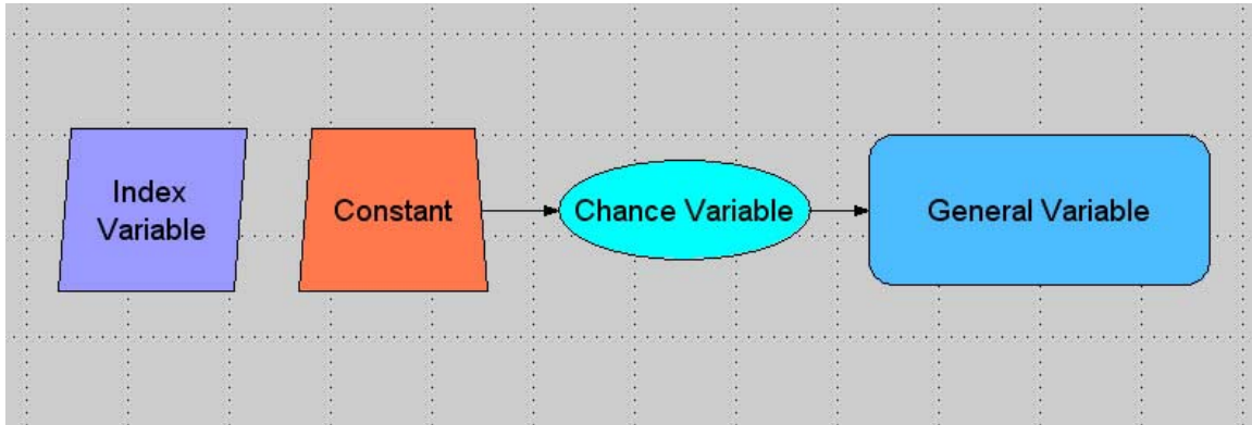
Figure 2.1: Analytica Diagram Window, showing from left to right an Index Variable Node, Constant Node, Chance Variable Node and General Variable Node. The Influence Arrows indicate that the Constant Node is included in the calculation of the Chance Variable Node, which in turn is included in the calculation of the General Variable Node. The presence of the Index Variable indicates that the model calculations are performed on a list of items.
